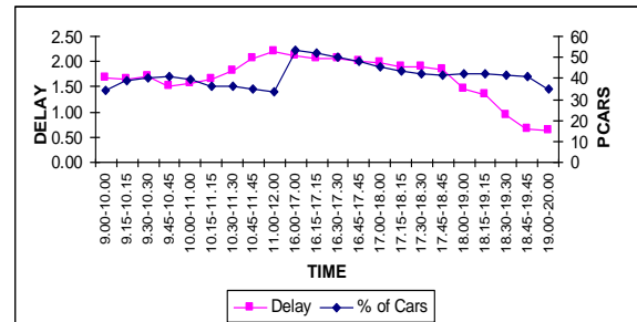
Figure 5.17: Delays vs. PCARS
