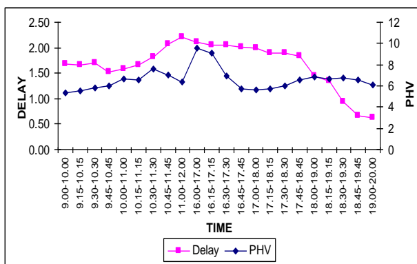
Figure 5.16: Delays vs. PHV
