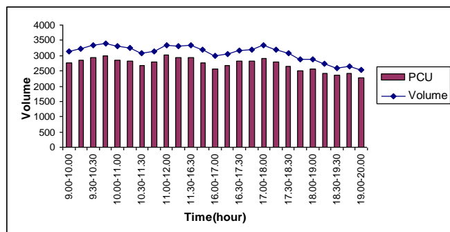
Figure 1.3: Peak hour volume for KVR Petrol bunk to Ayyappagudi junction
