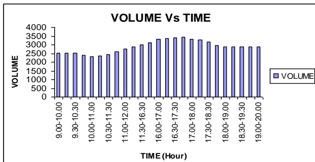
Figure 1.1: Peak hour volumes for KVR Petrol Bunk junction
