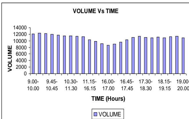
Figure 1.2: Peak hour volumes for Ayyappagudi junction
