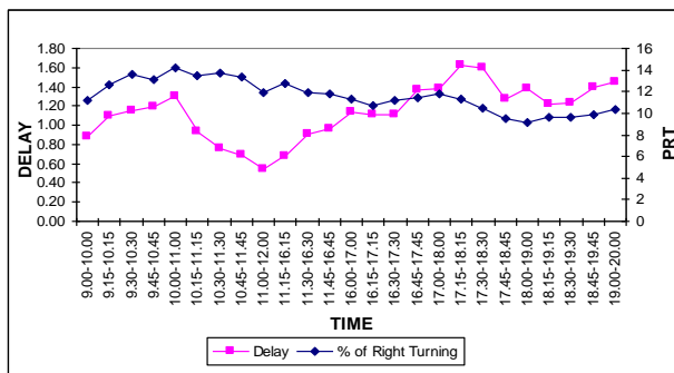
Figure 5.9: Delays vs. PRT
