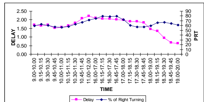
Figure 5.19: Delays vs. PRT
