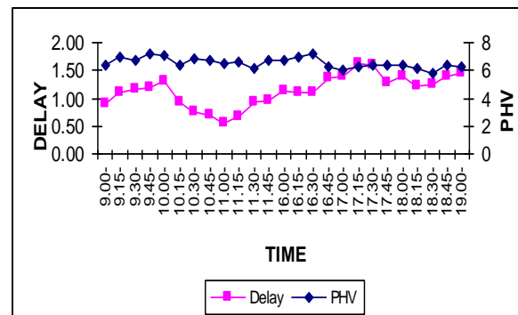
Figure 5.6: Delays vs. PHV
